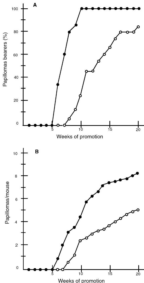
Figure 2. Inhibition of peroxynitrite/TPA-induced tumor promotion by multiple application of myricanone (2). (A) Percentage of mice bearing papillomas. (B) Average number of papillomas per mouse. ●, peroxynitrite (390 nmol) + TPA (1.7 nmol) (Group I); ○, peroxynitrite (390 nmol) + 0.0025% of 2 (2 weeks) + TPA (1.7 nmol) (Group II). At 20 weeks of promotion, the number of papillomas per mouse differed significantly ( p < 0.05) between Group I and Group II. The number (standard deviations are shown in parentheses) of papillomas per mouse for each group was 8.1 (1.9) and 5.0 (2.0) for Groups I and II, respectively.
