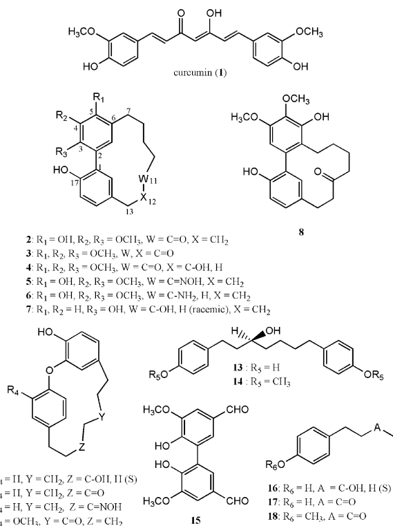
Figure 1. Structures of cyclic diarylheptanoids and derivatives.
